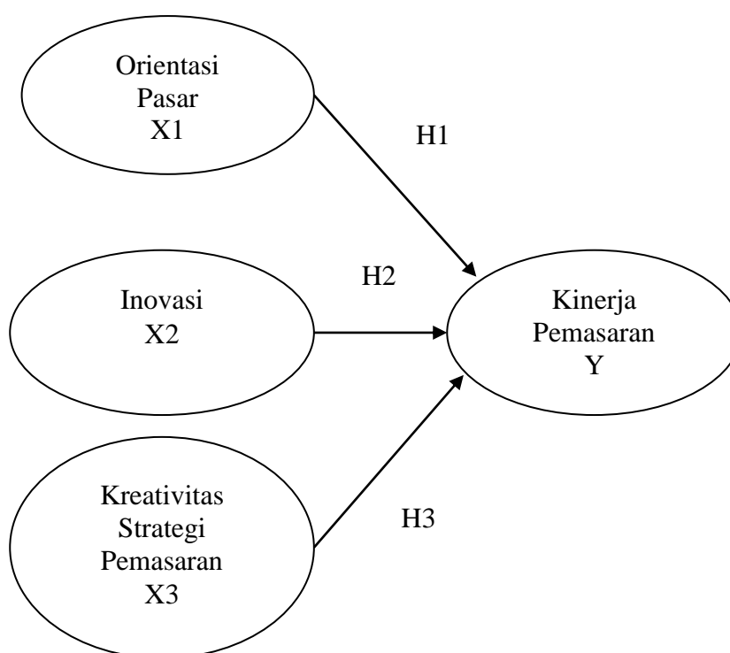
Gambar 1. Model Penelitian
