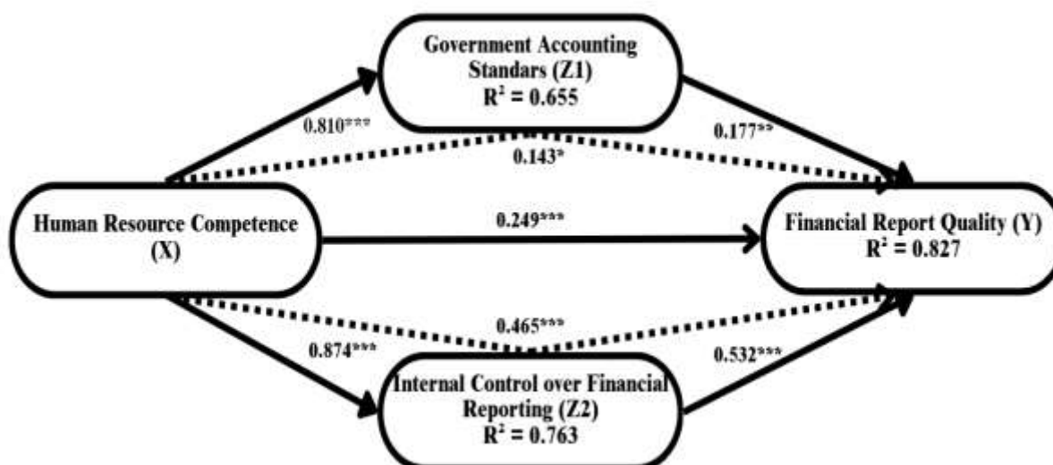
Figure 3. Result path diagram model – test of the main hypotheses.
